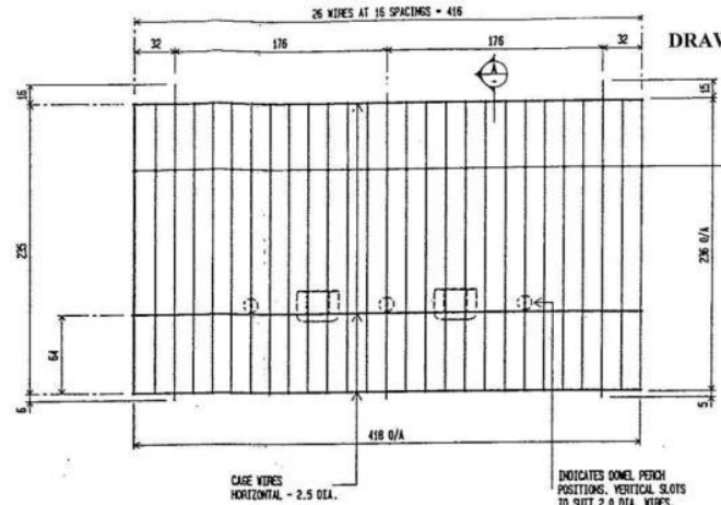
ELEVATION - WIRE CAGING
