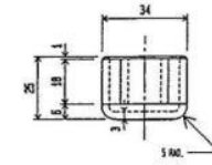
SECTION SCALE 2:1
